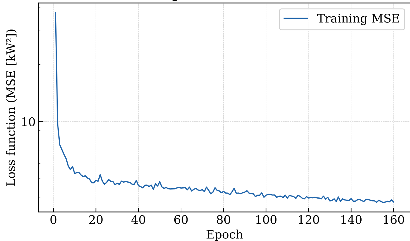
Learning curve — LSTM model
